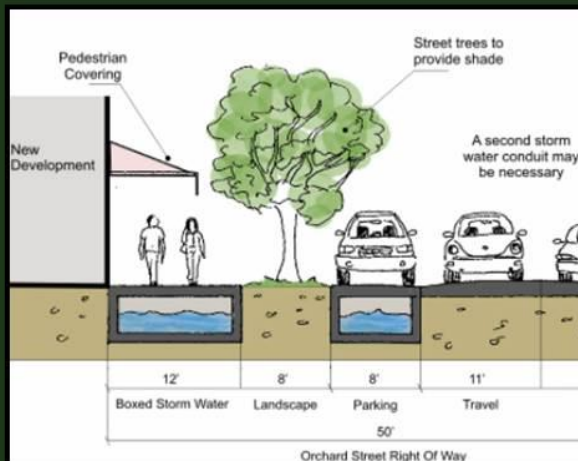
Conceptual sketch of a storm-water management retrofit for the Orchard Street/Fiesta Drainage. - Garapan and Beach Road Revitalization Plan, 2007
