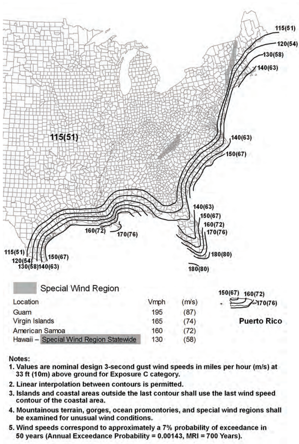
Figure 4-1 continued. Peak gust wind speeds in the United States. Source: Minimum Design Loads for Buildings and Other Structures , ASCE/SEI 7-10. Used with permission from ASCE.
